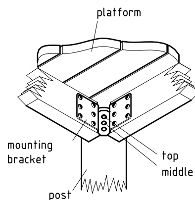
platform fastening 1:10
